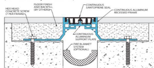
Fire Blanket System (101-A01-050 system shown)
