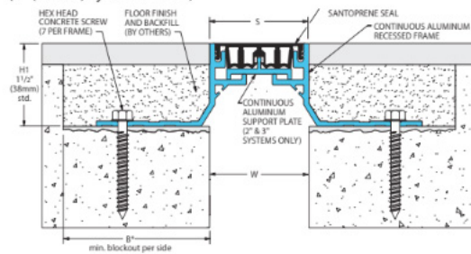
101-A01 Floor/Floor (2" (50mm) system shown)
