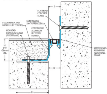
101-A02 Floor/Wall (1" (25mm) system shown)
