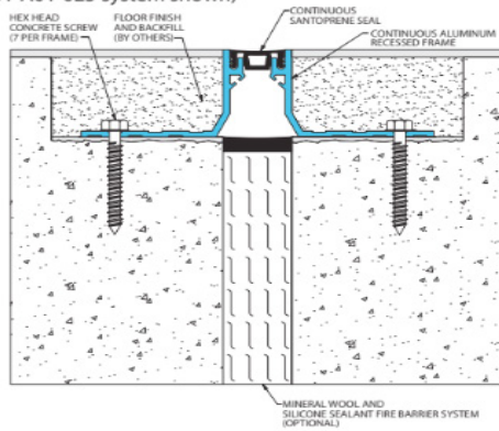
Mineral Wool & Sealant Fire Barrier System (101-A01-025 system shown)
